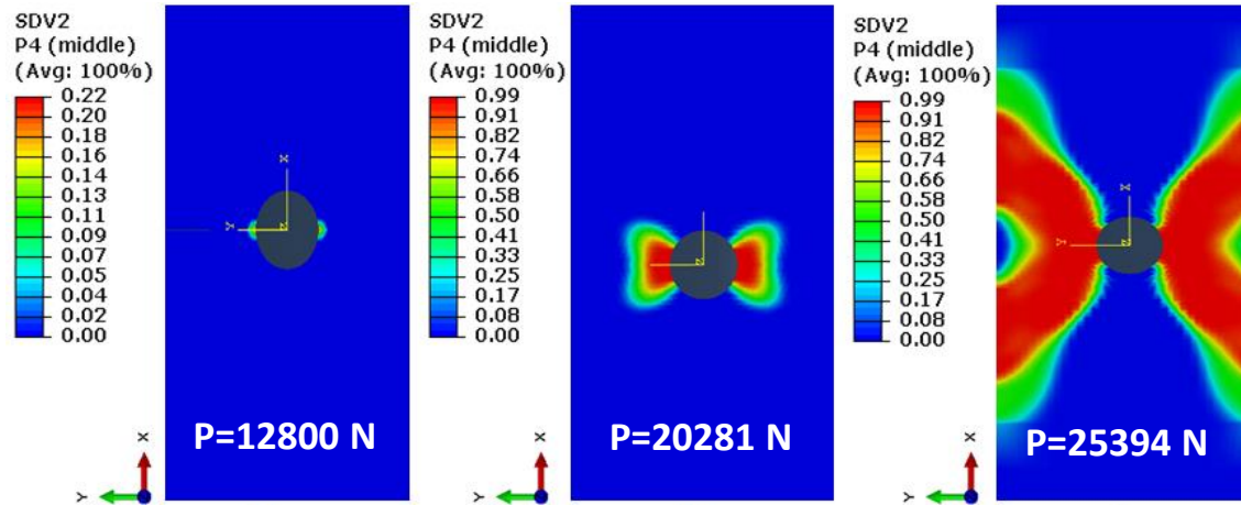
Matrix damage accumulation in 90° ply
