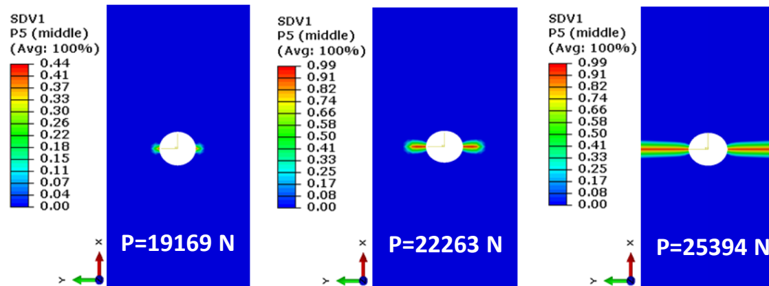
Fiber damage accumulation in 0° ply
